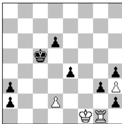
h # 9 (4 + 8) Circe, ABC inverse
