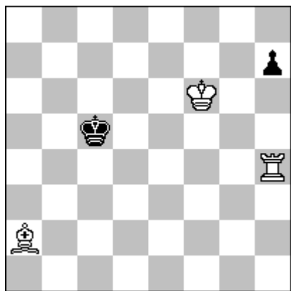
h # 14 (3 + 2) Mandatory black pursuit
