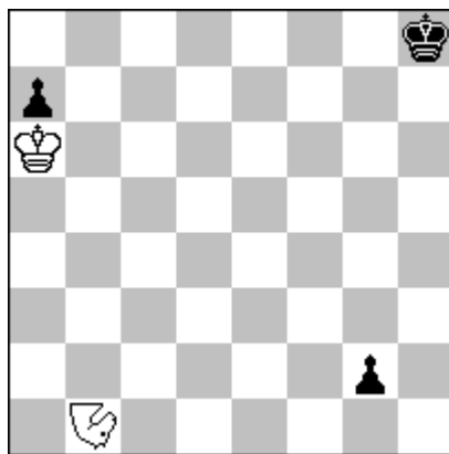
h # 19 (b1 - Tireur Knight/Camel) (2 + 3) Mandatory black pursuit
